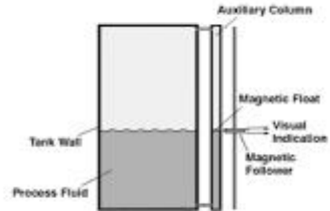
Magnetic level sensors
