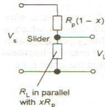
The circuit as a potential divider
