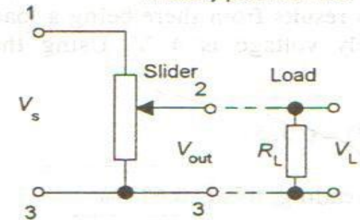
The circuit when connected to a load
