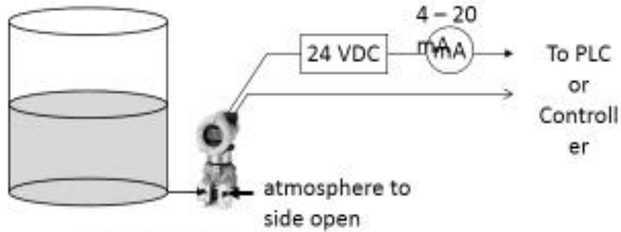
d/P Cell Transmitter
