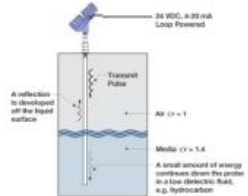
Radar level Sensors
